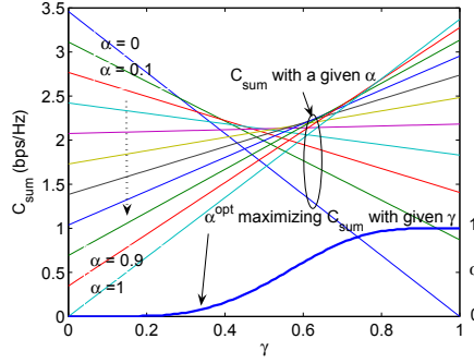
Fig. 2. C_{sum} with different \alpha and \gamma ( T_t = 1 , T = 1000 , \rho = 0.1 and P = P_2 = 10 dB)
