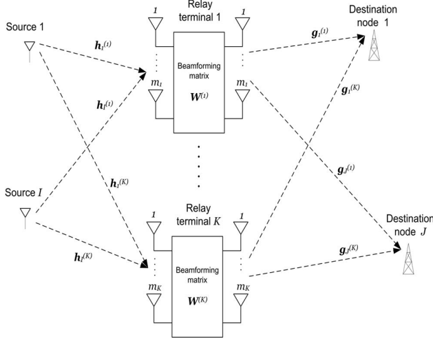
Fig. 1. System Model.
