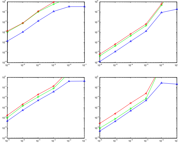
Fig. 1. Figures illustrating the effect on noise on the estimation of absolute time differences \triangle , microphone localization \triangleright and source localization \triangleleft . 3D sound-3D array localization (5s/10m and 20s/20m) (top) and 3D sound-2D array localization (5s/9m and 20s/20m) (bottom).
