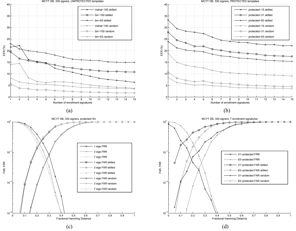
Fig. 2. Performance results of the template protection system for dynamic signature verification.
