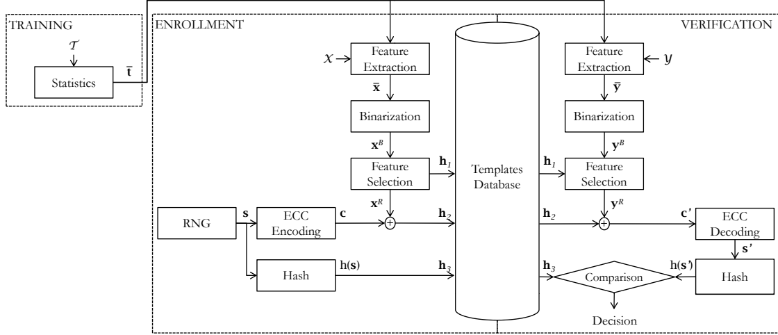
Fig. 1. Architecture of the helper data system, adapted from [5].
