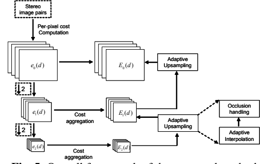
Fig. 5. Overall framework of the proposed method.
