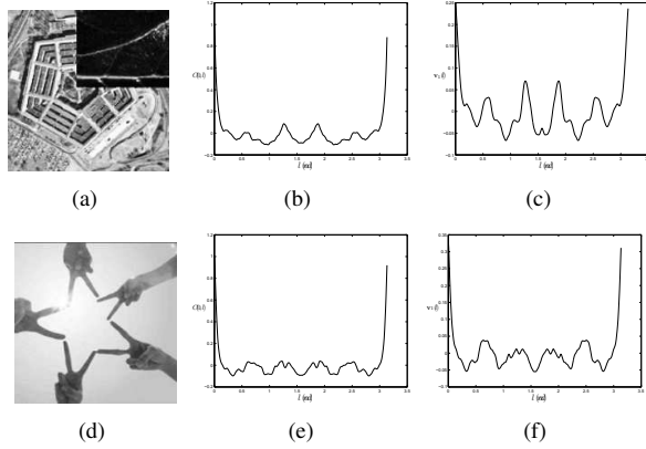
Fig. 1. (a)-(c): A corrupted symmetric image of order 5, the 1D autocorrelation C(0, l) and the periodic pattern v_1(l) extracted using SVD. (d)-(f): Another example of a non-perfect symmetry and the obtained C(0, l) and v_1(l) respectively.
