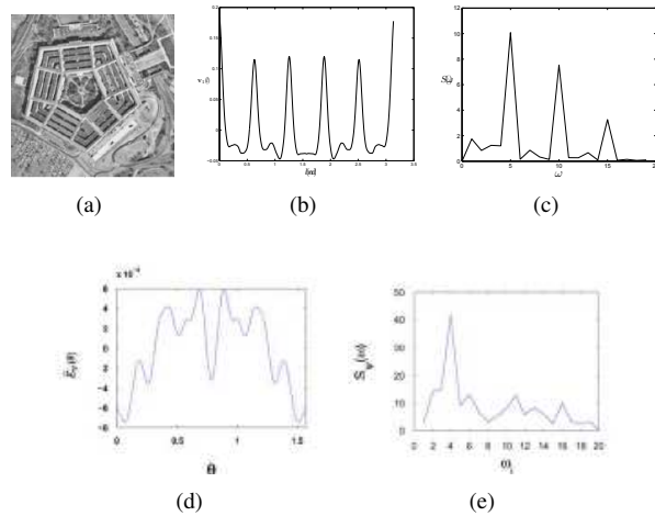
Fig. 2. (a): A non-perfect symmetry of order 5. (b)-(c) the periodic pattern v_1(l) extracted using SVD and its Fourier spectrum. (d)-(e): The periodic pattern extracted using the method in [3] and its Fourier spectrum.
