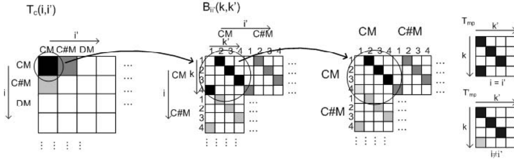
Fig. 1. Chord transition matrix for a singles-state HMM [left], transition matrices for Major to Major chords in the case of double-states HMM, without taking into account the pim of the chord in the measure [middle left] and taking into account the pim of the chord [middle right], pim transition matrices [right].
