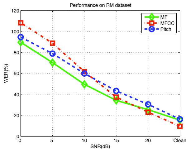
Fig. 4. Word error rates (WERs) obtained using the DARPA Resource Management Corpus, comparing speech separation using modulation frequency (MF), speech separation using pitch only (Pitch), and baseline MFCC processing without speech separation (MFCC).
