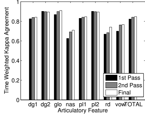
Fig. 3. Time-weighted Kappa for each pass through the manually transcribed SVitchboard utterances.
