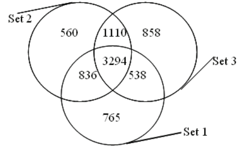
Fig. 2. Overlap between the 3 generated script sets. The circle “Set 1” denotes the script set of old corpus TH-CoSS. The circle “Set 2” denotes the script set designed by the rule-based tree method. The circle “Set 3” denotes the script set designed by our decision tree based method.
