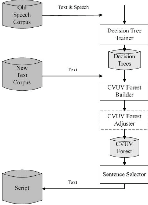
Fig. 1. Process flow of the proposed script design approach
