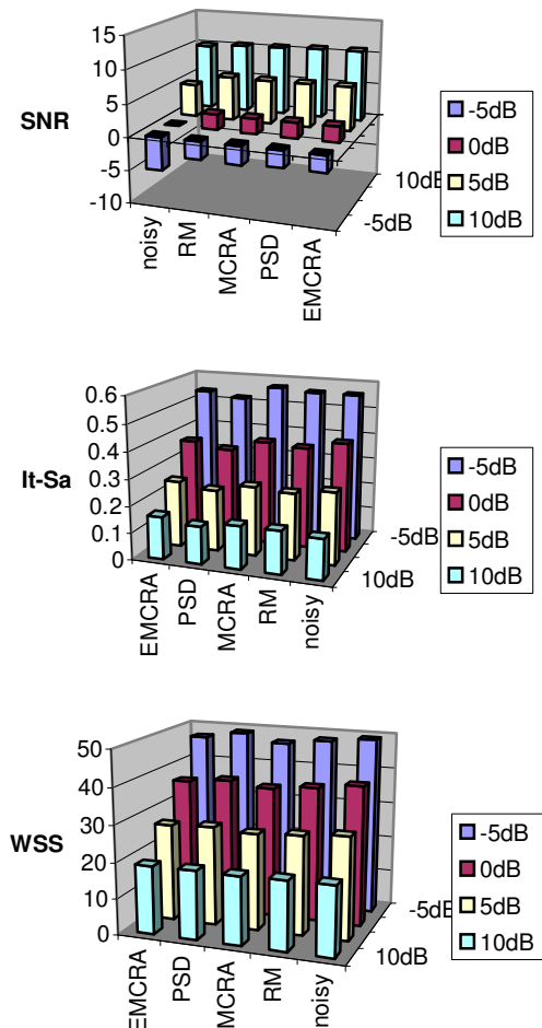
Figure 3 - Average filtered SNR (top), Itakura-Saito distortion (middle), and Weighted Spectral Slopes (bottom) scores at different input SNR for various noise estimators: RM [1], MCRA[2], PSD[5], and EMCRA.
