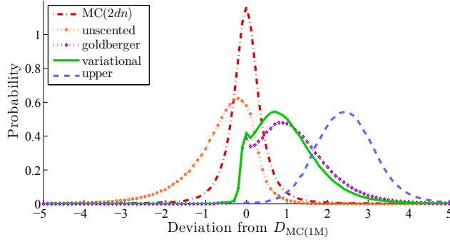
Fig. 2. Distribution of leading approximations to KL divergence relative to the reference estimate D_{MC(1M)} .
