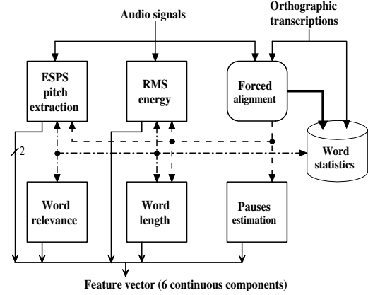
Fig. 1. Data flowchart of the feature extraction process.
