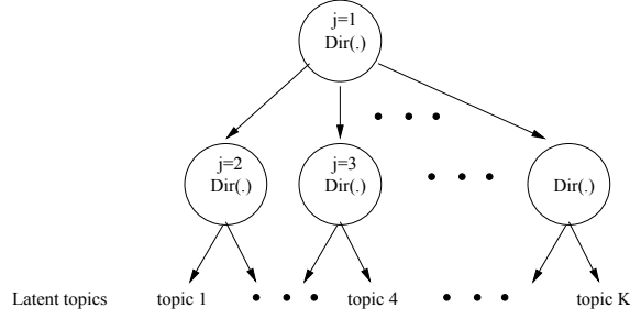
Fig. 1. Dirichlet-Tree prior of depth two: Each internal node is represented by a Dirichlet distribution over the branches.
