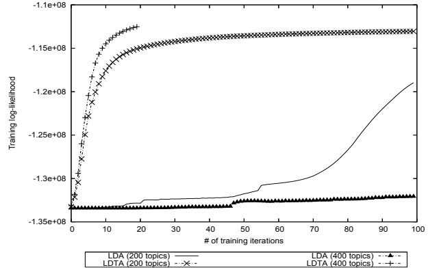
Fig. 2. Log-likelihood comparison of the LDA and LDТА models on the Xinhua News 2002 training corpus.
