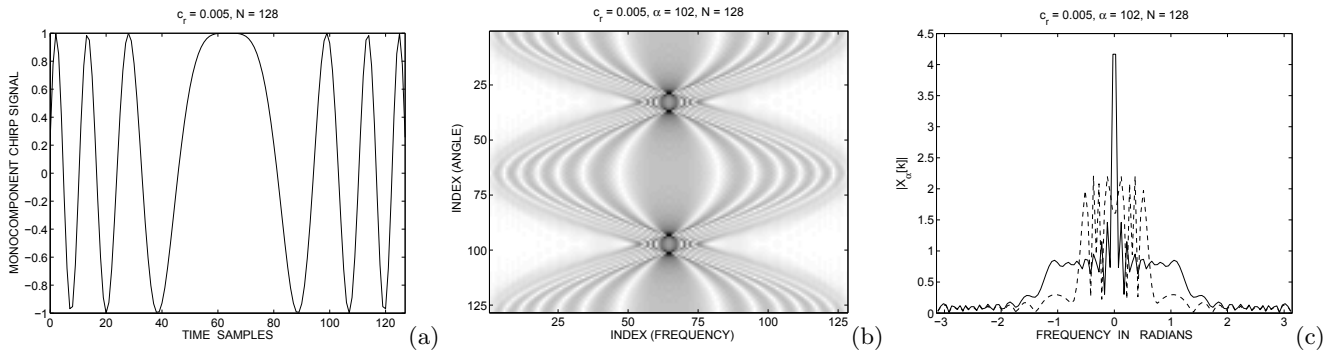
Figure 3: Concentrating a chirp: (a) chirp signal with a chirp rate of c_r = 0.005 and zero average frequency, (b) MA-CDFRFT of the chirp signal in (a), (c) cross-section of the MA-CDFRFT through the row containing the peak and the conventional CDFT.
