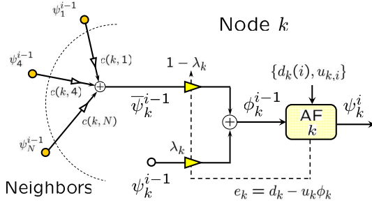
Fig. 3. A simple adaptive diffusion strategy.
