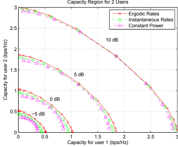
Fig. 1. 2-User capacity Region for ergodic capacity maximization, instantaneous capacity maximization, and constant power allocation.
