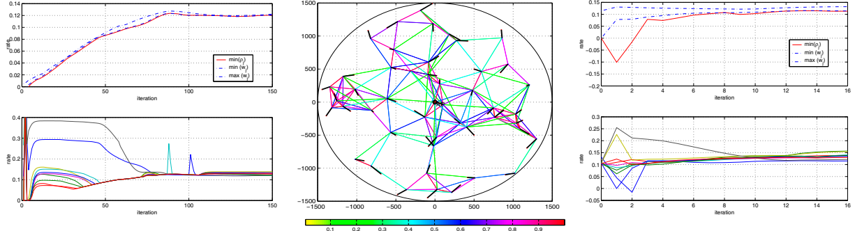
Fig. 3. Convergence of Algorithm 1 to the max-min optimal routes in Fig. 2 (left), and its response to user mobility (middle) and (right). After 70 iterations the rate of the most compromised user is within 90% of the optimal rate. The algorithm is fast to respond to changes in \mathbf{R} .
