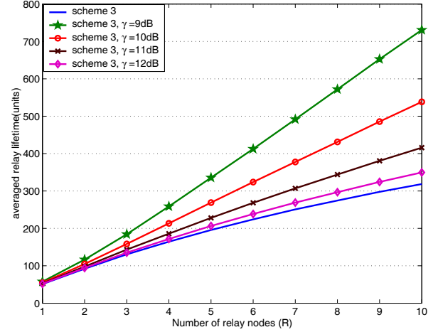
Fig. 4. The averaged relay lifetime of the opportunistic scheme with power saving as a function of the relay node number.
