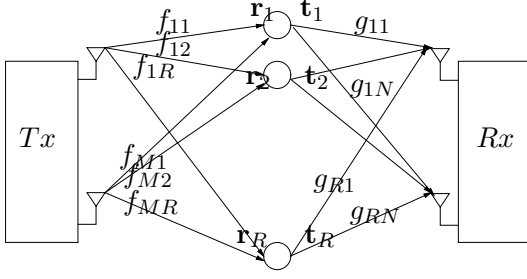
Fig. 1. The wireless network model with several antennas.
