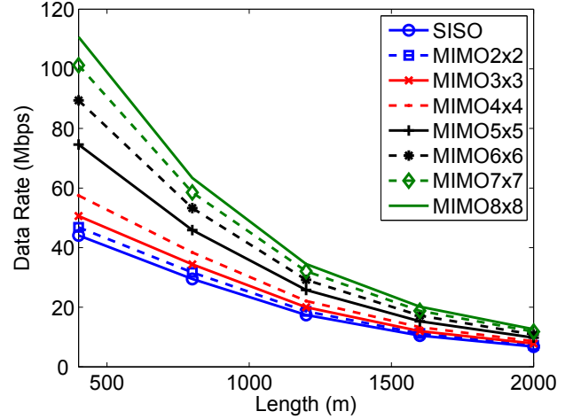
Fig. 1. Capacity per line with 2-sided coordination in a down-link scenario under per-modem total power constraints with spectral mask constraints
