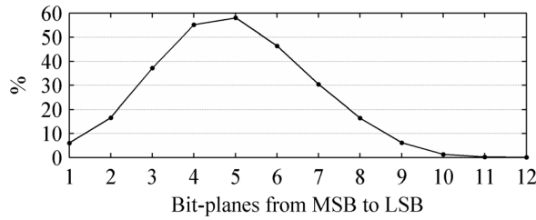
Fig. 6. Percentage of bits coded by the ZC primitive.
