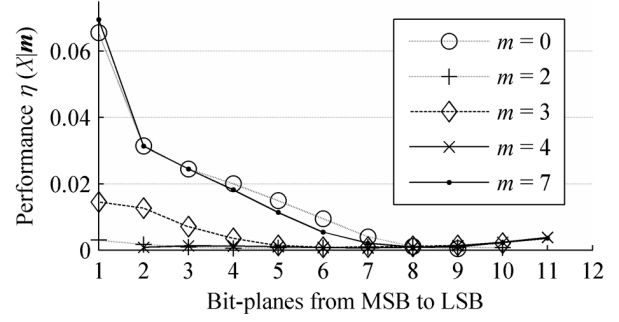
Fig. 2. Performance \eta(X, \mathbf{m}) of five ZC contexts in the LH and HL subbands of test set S1.
