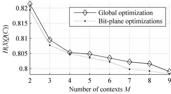
Fig. 3. Conditional entropies for different sets of optimal contexts.
