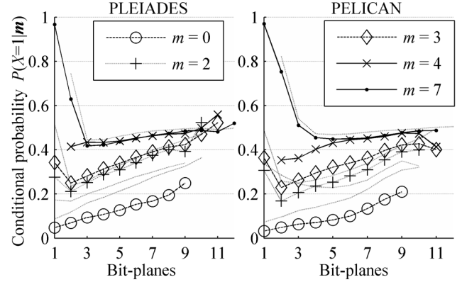
Fig. 4. Average conditional probabilities P(X = 1|m) of the ZC contexts on the sets of PLEIADES and PELICAN images.
