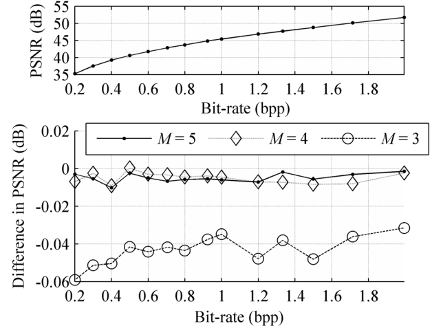
Fig. 7. Rate-distortion curve with JPEG2000 and difference of PSNR with combined contexts.
