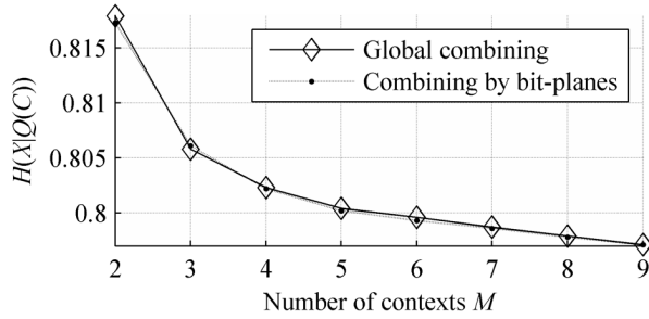
Fig. 5. Conditional entropies for different sets of merged contexts.
