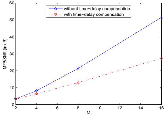
Fig. 1. \frac{MFB}{SNR_{out}} with and without relative time-delay compensation
