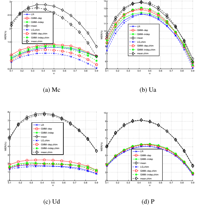
Fig. 2. WER versus \alpha (the lower the better) on (a) Mc (840 fusion sets \times 4 fusion operators), (b) Ua (840 \times 4 ), (c) Ud (840 \times 4 ) and (d) P (860 \times 4 ) protocols. The four fusion operators are: logistic regression (cross), GMM with dependent assumption (circle), GMM with independent assumption (asterisk) and the mean operator (diamond). Comparison should be made between a thin continuous line and a thick dashed line.
