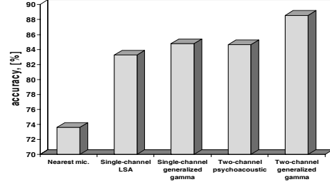
Fig. 3. Speech recognition overall performances on CIAIR in-car database
