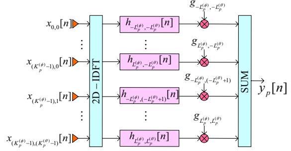
Figure 4. UCSA-FIB block diagram for the p^{\text{th}} sphere.
