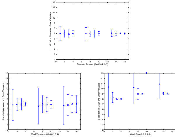
Fig. 4. Localization mean and error variance of 4 and 16 sensors at time of first detection ( * and \circ ) and after accruing information ( \triangle and \diamond ) for three values of release amount (top), unmodeled wind variance (bottom left), and unmodeled wind bias (bottom right).
