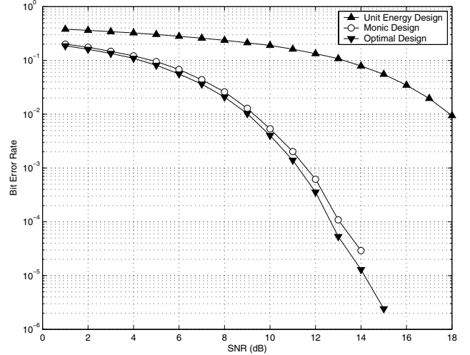
Fig. 1. Comparison of BER performance of three designs.
