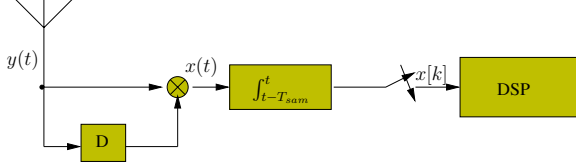
Fig. 1. Autocorrelation receiver
