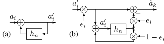
Fig. 2. (a) Transmitter and (b) receiver structure projecting erasure errors. Only the receiver is aware of the erasure.
