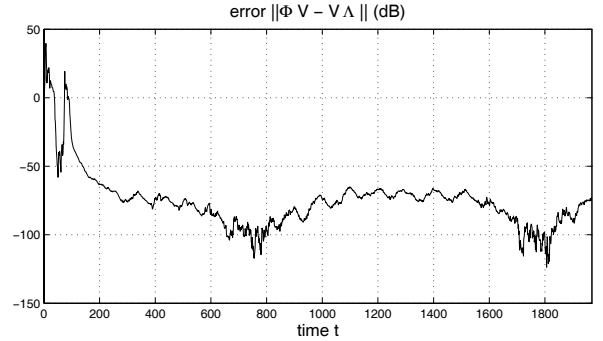
Fig. 2. Representation of the error \|\Phi(t)\mathbf{V}(t) - \mathbf{V}(t)\Lambda(t)\| in the coupled estimation of the eigenvalues matrix \Lambda(t) and the eigebasis \mathbf{V}(t) .
