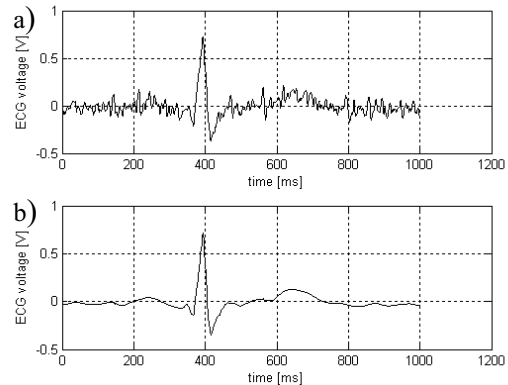
Fig. 5: Denoising method applied on ECG affected by physical sources of noise: the acquired signal (a) and the processed signal (b).
