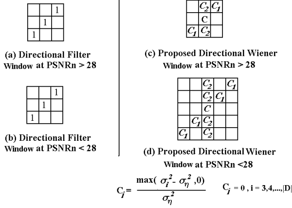
Fig. 2. Fixed directional filter versus proposed variable kernel shape and direction at different noise levels.
