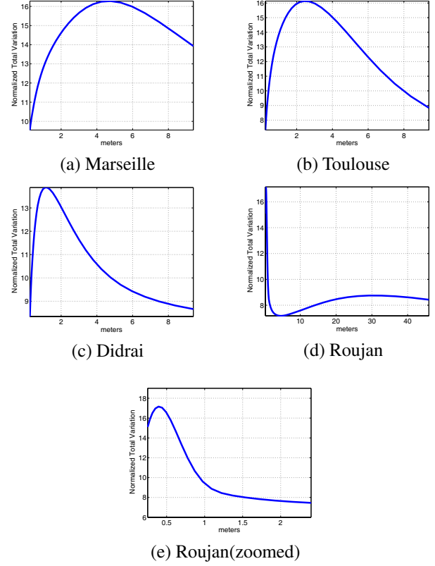
Fig. 3. (a) NTV computed on the image of Marseille ( r = 0.25m ); t_{\max} = 4.8m ; (b) NTV computed on the image of Toulouse ( r = 0.25m ); t_{\max} = 2.4m ; (c) NTV computed on the image of Didrai ( r = 0.25m ); t_{\max} = 1.2m ; (d) NTV computed on the image of Roujan ( r = 0.25m ); there are two local maxima. The first one appears at the resolution 0.4m , the second one appears at the resolution 30m ; (e) Zoom around the first local maximum shown in (d).
