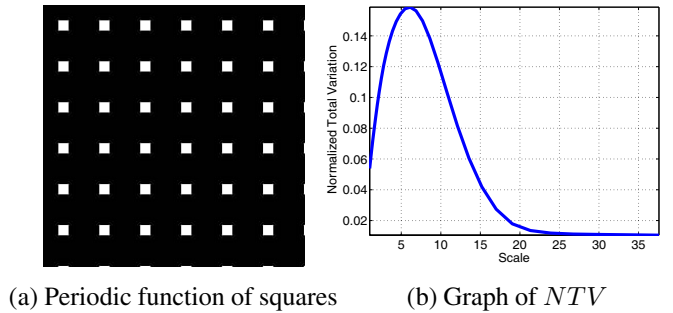
Fig. 1. An image composed of squares with spatial period D = 40 (the length of each square being 10 pixels) and the graph of the normalized total variation. The maximum is reached for t = 6.1 .
