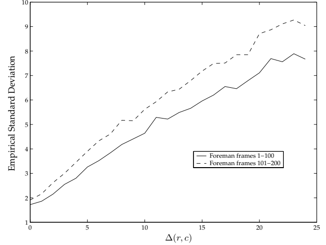
(b) Empirical standard deviation conditioned to \Delta(r, c) on foreman.
