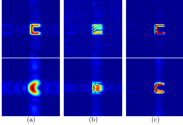
Fig. 3. Reconstructed images from full-aperture data. (Magnitudes shown.) Top: 730 kHz. Bottom: 300 kHz. (a) Beamforming. (b) Regularized pseudoinverse. (c) Proposed method.
