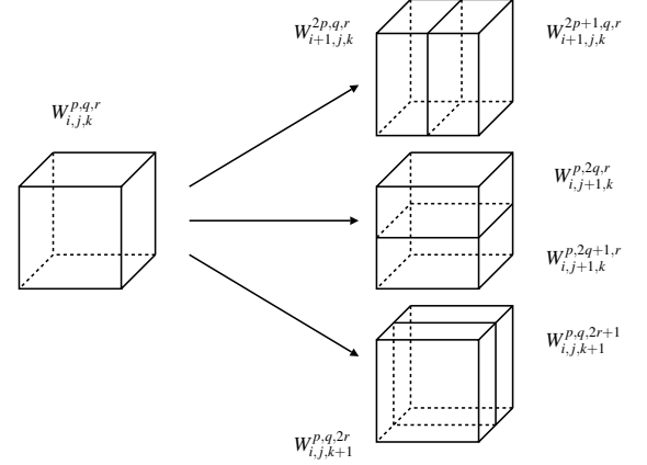
Fig. 2. Anisotropic decomposition and notations.
