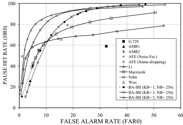
Fig. 3. ROC curves obtained in high noise conditions.
