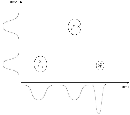
Fig. 4. GLDA clustering plot for n = 2 , p(1) = 1 , p(2) = 1 , M(1) = 3 and M(2) = 2 .
