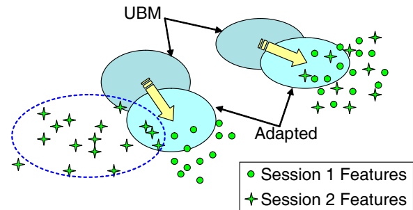
Fig. 1. MAP adaptation for incomplete data. This example demonstrates features that do not obey the identically distributed assumption across audio sessions.
