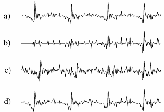
Fig. 2. Example of a resynchronized excitation: (a) the correct excitation, (b) the excitation e_0(n) , (c) the excitation signal built using the erroneous ACB memory and (d) the excitation signal built after correcting the ACB memory.
