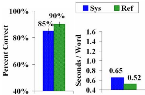
Figure 3: Conventional STT Transcript Readability
