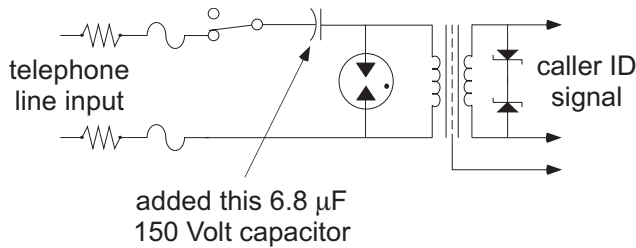
Fig. 2. Schematic diagram of the modified telephone coupler, with the added capacitor shown.
