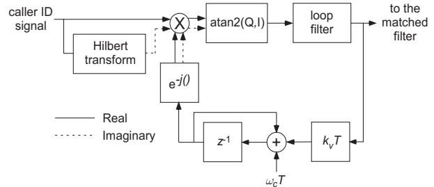
Fig. 4. Block diagram of the FSK demodulator.
