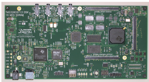
Fig. 6. A Texas Instruments TMS320C6713 DSP Starter Kit (DSK).
