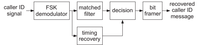
Fig. 3. Block diagram of the caller ID system.
