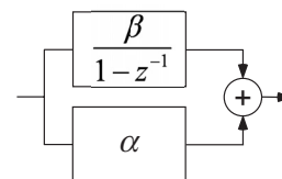
Fig. 5. Block diagram of the FSK demodulator's loop filter.
