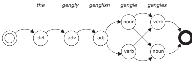
Fig. 3. An example of a lattice bigram for a simple Genglish sentence. Transition probabilities are associated with arcs. Each state is capable of emitting the word it refers to with a state-dependent emission probability.
