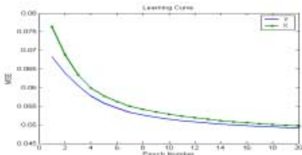
Figure 3. Learning curve
