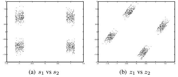
Fig. 1. Scatter plots (a) of the bimodal sources \mathbf{s} and (b) of the whitened signals \mathbf{z} ; \phi = \pi/6 .
