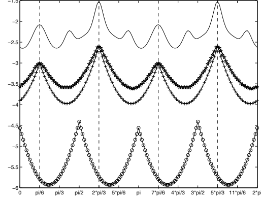
Fig. 2. Contrasts \mathcal{C}^2 (+), \hat{\mathcal{C}}^2 (*), -H(y_1) (-) and function \bar{\mathcal{C}}^2 (o) vs \varphi . The only relevant maxima are located at \varphi = \pi/6 + k\pi/2 ( k \in \mathbb{Z} ) ( \phi = \pi/3 );
