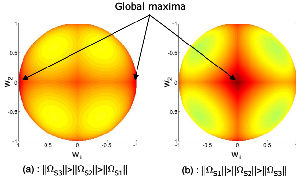
Fig. 3. Manifold of the contrast function \hat{\mathcal{C}}^3 projected on the 2D space w_1, w_2 .
