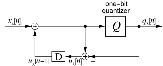
Fig. 1. A basic \Sigma\Delta modulator using (I.6) and (I.7).
