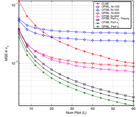
Fig. 2. MSE in \mathbf{v}_1 vs L , 4 \times 4 system, for two different values of N , and data and training symbol SNR fixed at P_T = P_D = 10\text{dB} . The two competing semi-blind techniques, OPML and CFSB, are plotted. For finite N , CFSB outperforms OPML as it only requires an accurate estimate of \mathbf{u}_1 from the blind data.
