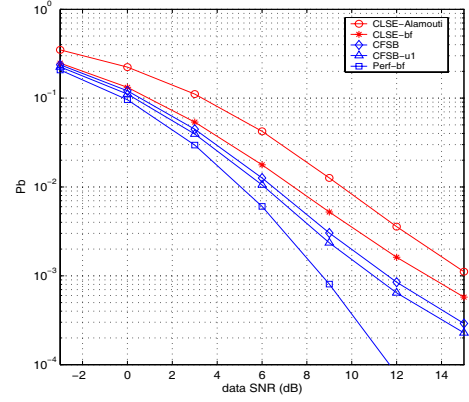
Fig. 3. Bit error probability versus data SNR for the 2 \times 2 system, with L = 2 , N = 16 , \gamma_p = 2\text{dB}
