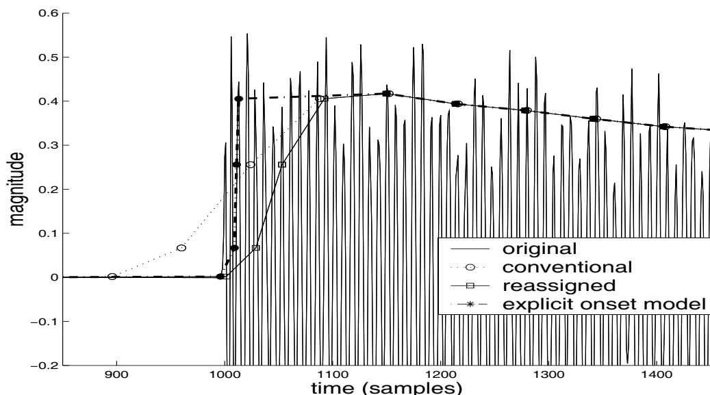
Fig. 5. Glockenspiel test signal with various model envelopes
