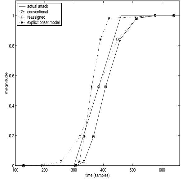
Fig. 4. Linear onset sinusoidal test signal: original envelope and detected envelopes.
