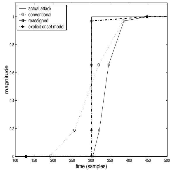
Fig. 2. Sinusoidal test signal: original envelope and detected envelopes.
