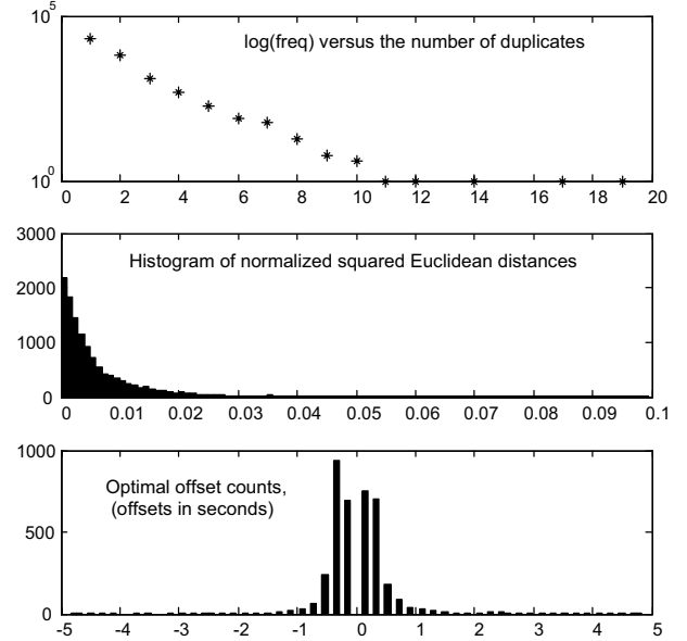
Fig. 2. Results of duplicate detection on 40,991 audio files.
